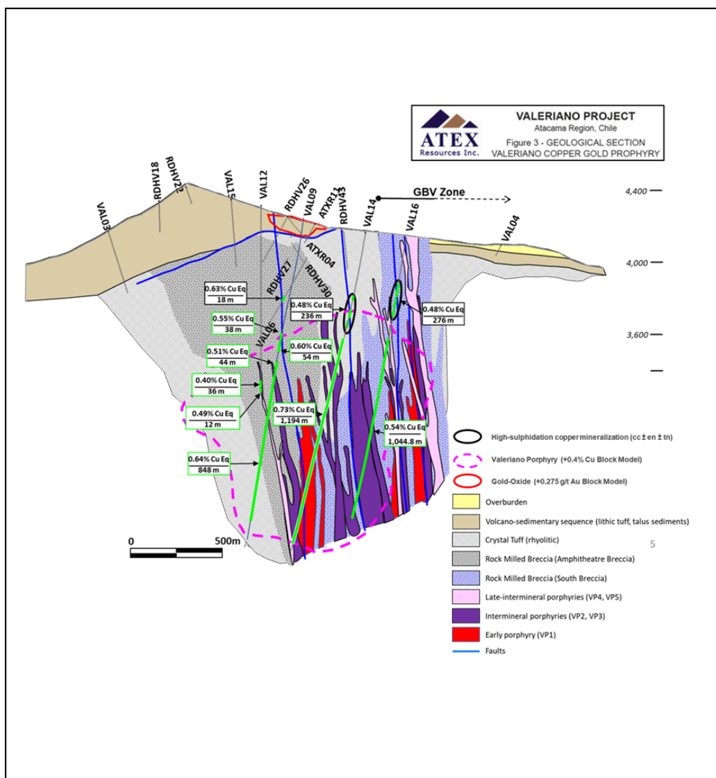
Figure 2 – Geological Section, Valeriano Copper Gold Porphyry
